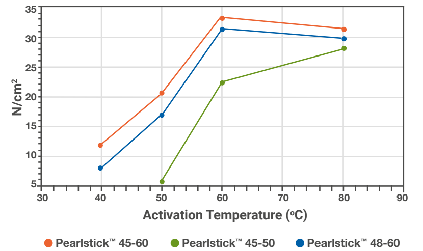
Hot-Tack 1 (PVC/Split leather) (Pressure: 2 kg/cm 2 , Contact time: 4 sec)
