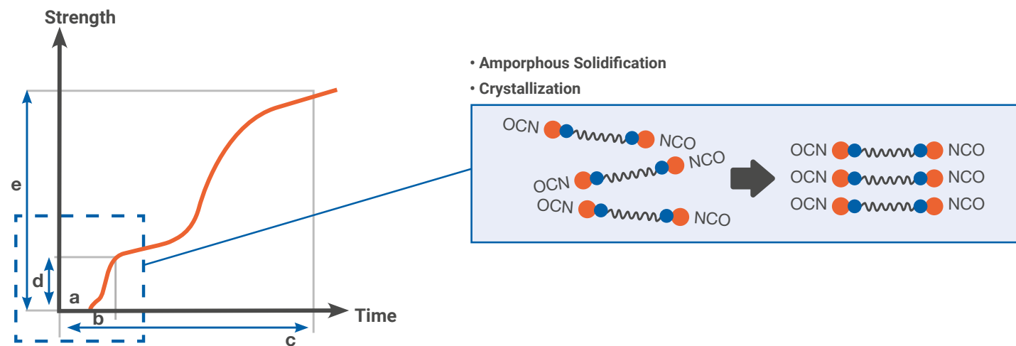
Figure 2. Physical crosslinking
